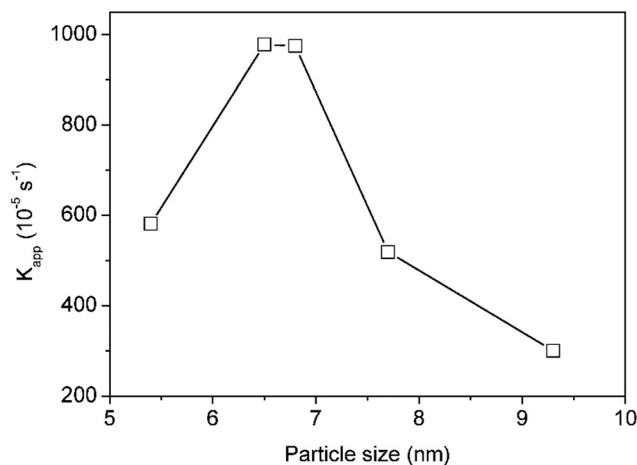
Fig. 13 Relationship between particle size and catalytic activity. Reaction conditions: 3.3 \times 10^{-5} \text{ M} 4-NP, 6.6 \times 10^{-2} \text{ M} NaBH 4 and 2.24 \times 10^{-5} \text{ g L}^{-1} silver nanoparticles at room temperature.
