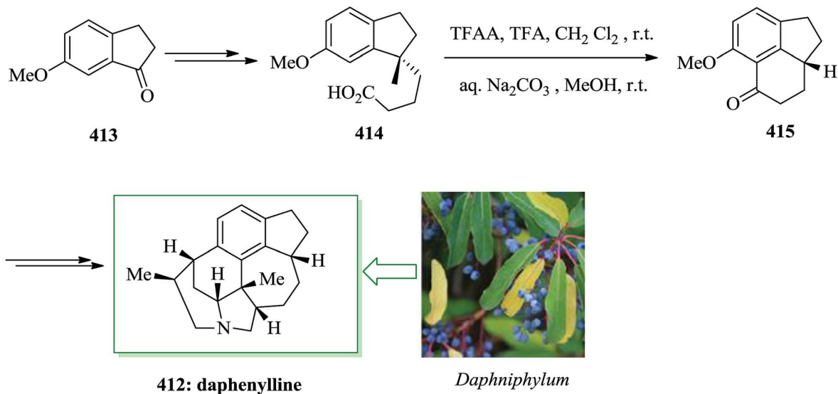
Scheme 77 Total synthesis of daphenylline 412.
