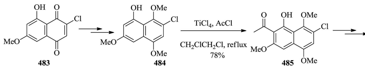
Scheme 102 Total synthesis of protein tyrosine phosphatase 1B (PTP1B).
