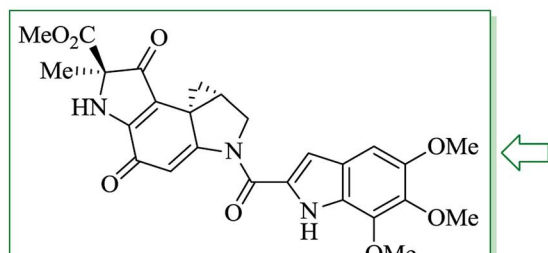
436: Duocannycin A
