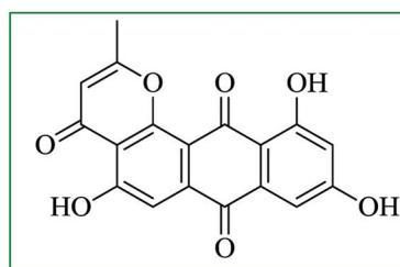
482c: Topopyrone C
