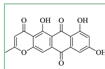
482d: Topopyrone D
