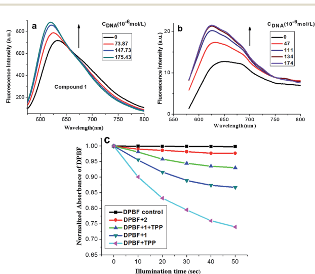
Fig. 2 Fluorescence spectra of compound 1 (a) and 2 (b) with the titration to ct-DNA. Each spectrum was recorded in pH = 7.4, 0.05 \text{mol L}^{-1} Tris-HCl, 0.1 \text{mol L}^{-1} NaCl buffer solution. (c) Singlet oxygen generation of 1 and 2 (50 \mu\text{M} ). The change of absorption of DPBF at 418 nm ( A/A_0 ) upon the irradiation time. The spectrum was recorded in DMSO.
