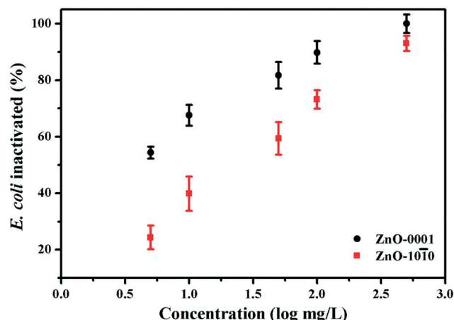
Fig. 9 Antibacterial activity of ZnO-0001 and ZnO-1010 nanomaterials under simulated solar irradiation. Error bars represent \pm one standard deviation from the mean ( n = 3 ).
