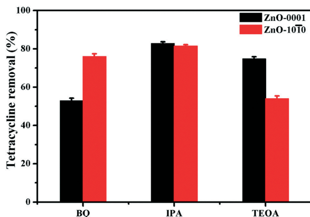
Fig. 8 Photodegradation of tetracycline by ZnO-0001 or ZnO-1010 in aqueous solutions with or without radical scavengers, after irradiation under simulated solar for 3 h. The 1,4-benzoquinone (BQ), isopropyl alcohol (IPA), triethanolamine (TEOA) were used as scavengers of O_2^{\cdot-} , HO^{\cdot} and h^+ , respectively. Error bars represent \pm one standard deviation from the mean ( n = 3 ).
