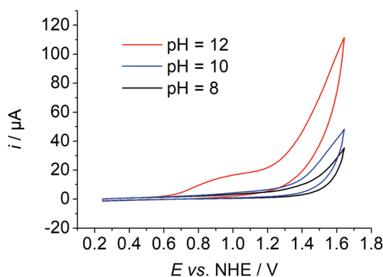
Fig. 2 pH dependent CV data of 1 in Millipore water ( [\mathbf{1}] \approx 1 mM, l = 0.1 M \text{PO}_4^{3-} , v = 0.1 \text{ mV s}^{-1} ).
