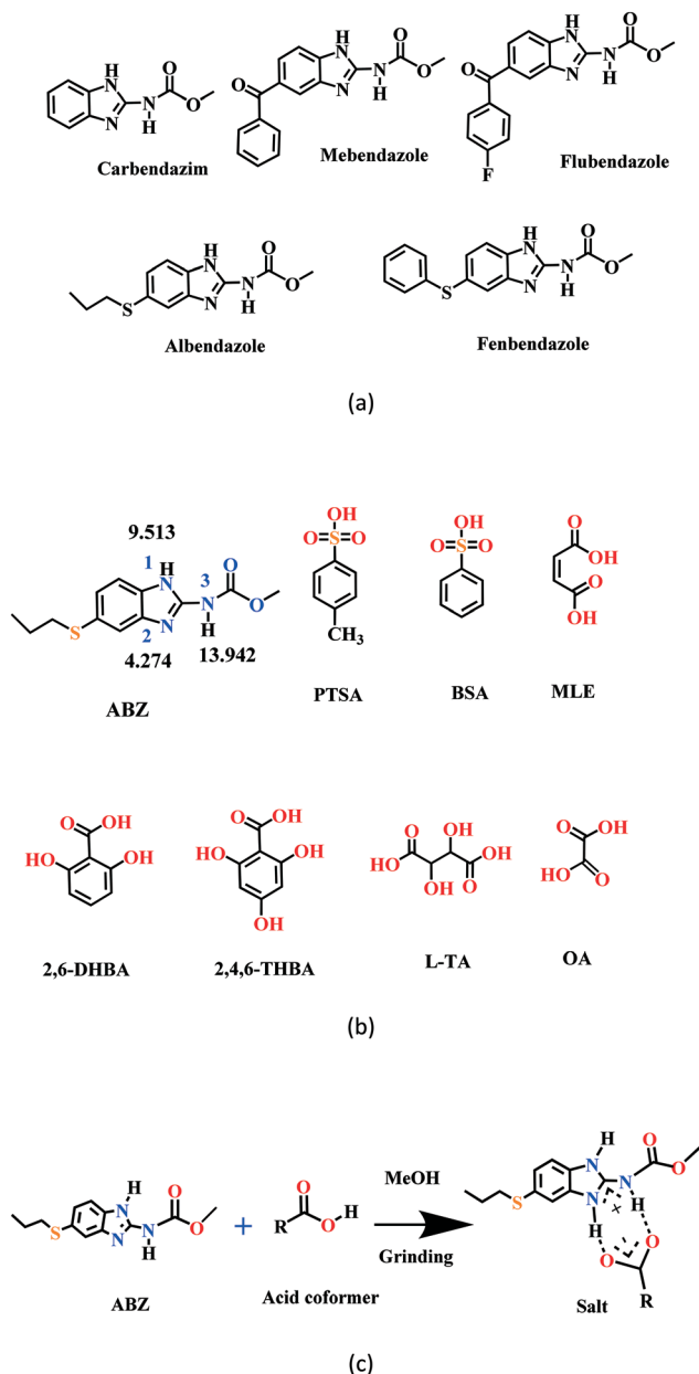
Scheme 1 (a) A few benzimidazole drugs. (b) Chemical structures of ABZ (along with their N pK_a values, will be discussed in later sections) and the cofomers reported in this study. (c) Ionic synthon of ABZ with carboxylic acid in an R_2^2(8) motif.
