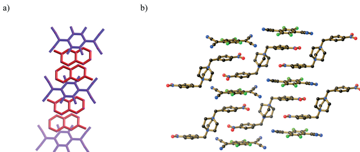
Fig. 21 a) A single type VI stack in (Meiq) 2 F 4 TCNQ (114), in which pairs of Meiq + cations (red) make face-to-face contacts with the F 4 TCNQ 2- anions (purple). b) A view of the crystal packing of (dnbdab)F 4 TCNQ (116) in which type VI stacks are linked by dnbdab cations.
