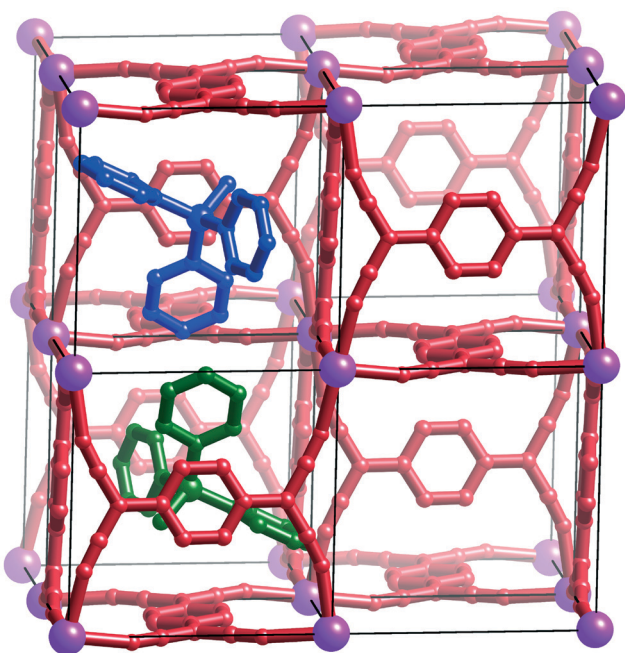
Fig. 11 A representation of (\text{MePPh}_3)_2[\text{Cd}_{12}(\text{TCNQ})_3] (64) illustrating the pseudo-cubic arrangement of Cd centres. For clarity, only two MePPh 3 + cations, which occupy "octants" within the framework are shown.
