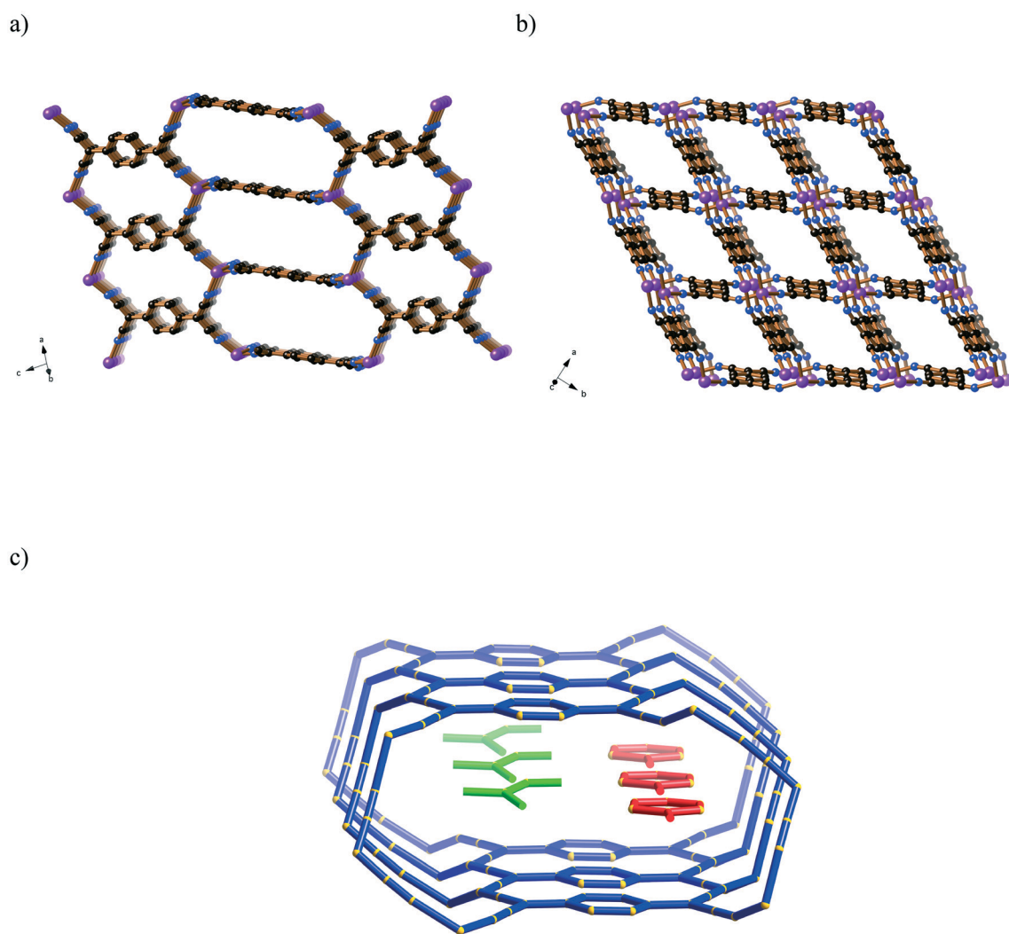
Fig. 16 The distorted [\text{Cu}^{\text{I}}(\text{TCNQ})]^- network in (\text{Mepyz})[\text{Cu}^{\text{I}}(\text{TCNQ})] (86) viewed a) slightly off the b axis and b) slightly off the pseudo-tetragonal axis. The Me-pyrazinium cations have been omitted. c) View along a single hexagonal channel in (\text{Mepyz})[\text{Cu}^{\text{I}}(\text{TCNQ})] occupied by \text{Mepyz}^+ cations (red) and DMF molecules (green).
