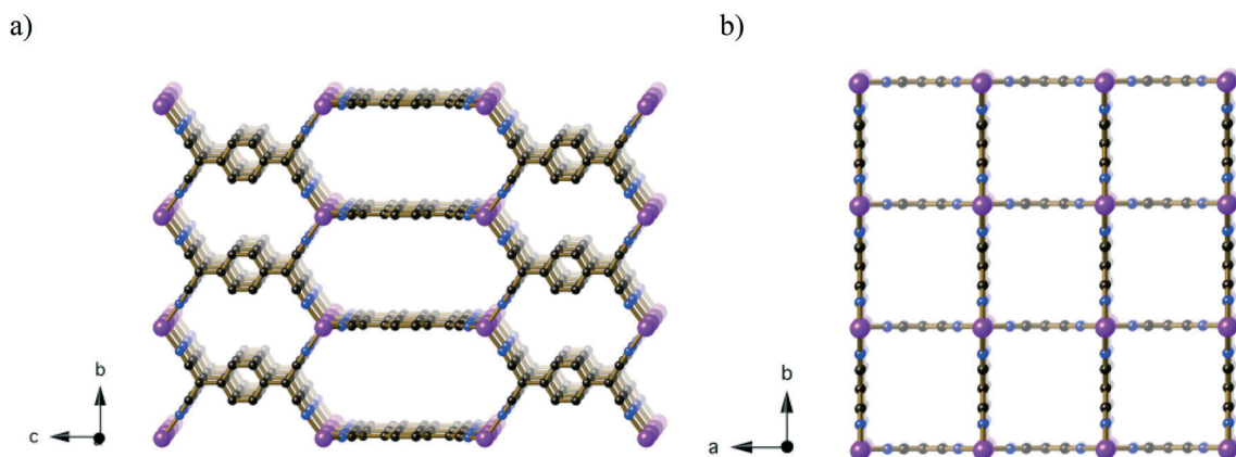
Fig. 15 The high symmetry [\text{Cu}^{\text{I}}(\text{TCNQ})]^- network in (\text{NMe}_4)[\text{Cu}^{\text{I}}(\text{TCNQ})] (81) viewed a) down the a axis and b) along the unique tetragonal axis. The \text{NMe}_4^+ cations have been omitted.
