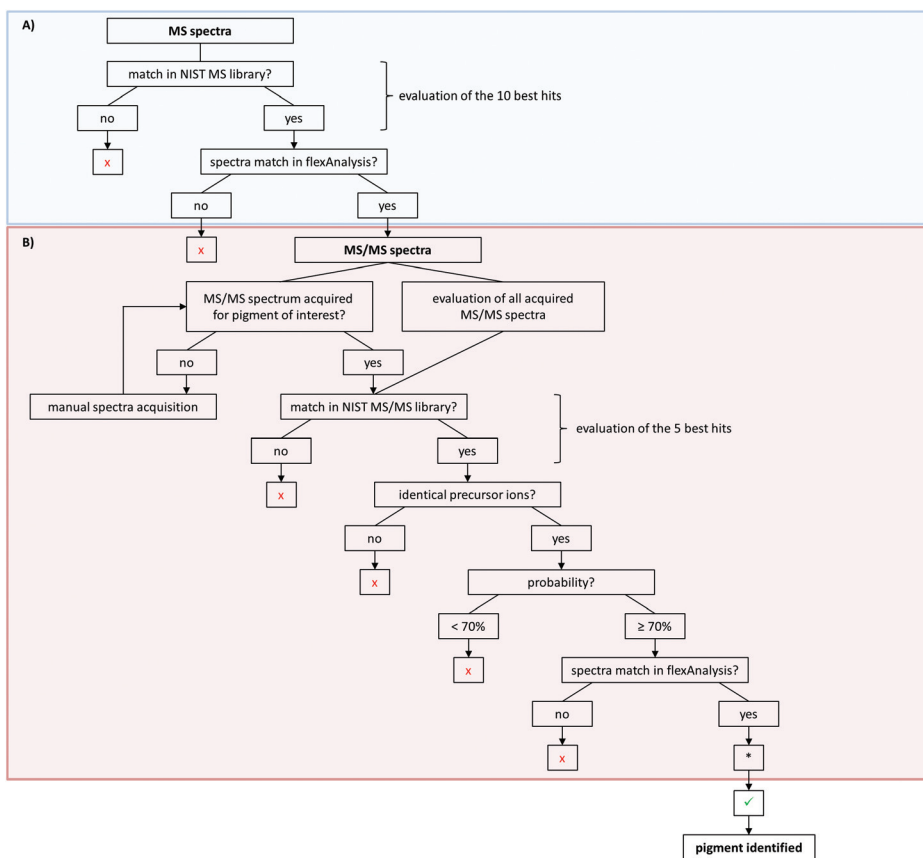
Fig. 4 Decision tree for pigment identification with NIST MS Search. (A) Evaluation of MS spectra. Spectra are considered to match if the molecular peak of the suggested library pigment or a high abundant fragment peak is present in the sample spectrum. (B) Analysis of MS/MS spectra upon successful or equivocal MS evaluation. If multiple similar spectra of the same pigment appear as best hits, the probability might be lower than 70% in rare cases. Evaluation of lithium-MS spectra is carried out analogously to MS analysis. x = pigment suggestion has to be turned down; ✓ = pigment suggestion can be accepted. *In cases where the MS/MS spectra analysis results in the suggestion of a pigment that was not found following the path of the MS spectra analysis, the MS spectrum has to be manually inspected for the corresponding pigment peaks.
