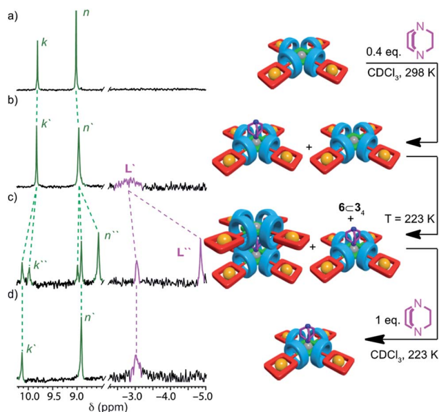
Fig. 3 Partial 1 H NMR (CDCl 3 , 300 MHz) of (a) pentad [5]rotaxane 6C34 (298 K); (b) 6C34 + DABCO (0.4 equiv., 298 K); (c) 6C34 + DABCO (0.4 equiv., 223 K); (d) 6C34 + DABCO (1 equiv., 223 K). Peak assignments as shown in Scheme 1. Primed (') and doubly primed labels refer to signals attributed to [(6C34)L] and [(6C34) 2 L] respectively. Cartoon representations have been included to aid clarity but are not intended to be representative of the structures of the complexes formed. 28
