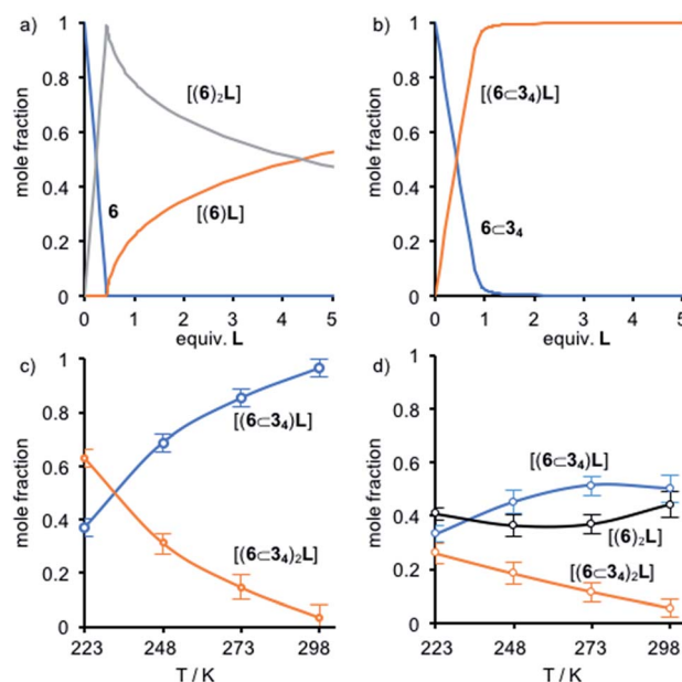
Fig. 4 Speciation diagrams for (a) 6 with respect to equiv. L; (b) 6C34 with respect to equiv. L; (c) L in a 6C34 + 0.4 L mixture with respect to T; (d) L in a 6 + 6C34 + L (1 : 1 : 1) mixture with respect to T.
