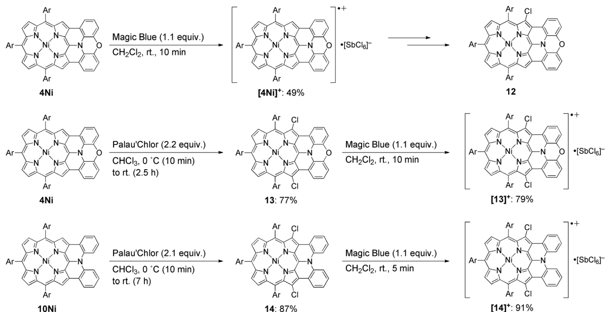
Scheme 2 Synthesis of radical cations [4Ni]^{\bullet+} , [13]^{\bullet+} , and [14]^{\bullet+} . Ar = 3,5-di- tert -butylphenyl.
