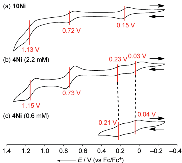
Fig. 5 Cyclic voltammograms of (a) 10Ni , (b) 4Ni at 2.2\text{ mM} , and (c) 4Ni at 0.6\text{ mM} . The redox potentials were measured by cyclic voltammetry in anhydrous \text{CH}_2\text{Cl}_2 with 0.1\text{ M} n\text{Bu}_4\text{NPF}_6 as a supporting electrolyte, and \text{Ag}/\text{AgClO}_4 as a reference electrode. The ferrocene/ferrocenium ion couple was used as an external reference. Scan rate: 0.05\text{ V s}^{-1} .
