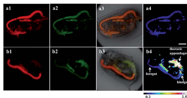
Fig. 8 Time-gated luminescence images of Daphnia magna treated with the RTLNP ( 100 \mu\text{g ml}^{-1} ) for 1.5 h (a), followed by incubation with HClO ( 50 \mu\text{M} ) for 20 min (b) (1: the images at the red channel; 2: the images at the green channel; 3: overlap of luminescence and bright-field images; 4: I_{\text{green}}/I_{\text{red}} ratiometric images). Scale bar: 200 \mu\text{m} .
