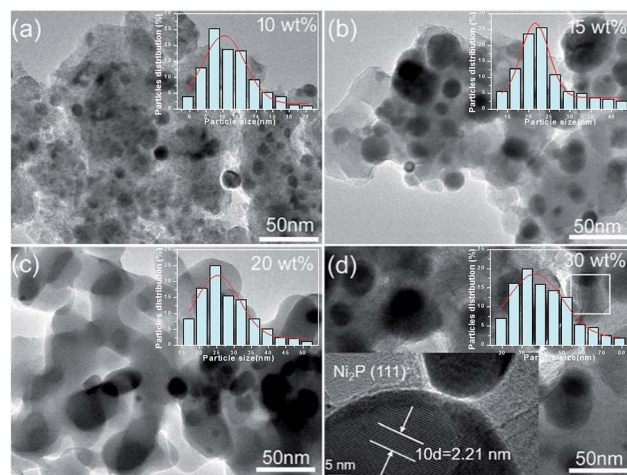
Fig. 3 The TEM images of \text{Ni}_x\text{P}-\text{Al}-\text{M} catalysts synthesized at 650^\circ\text{C} from \text{Ni}(\text{NO}_3)_2 \cdot 6\text{H}_2\text{O} and \text{NH}_4\text{H}_2\text{PO}_4 precursors with a mole ratio of \text{Ni}/\text{P} = 1.25 , and with different loadings: (a) 10 wt%, (b) 15 wt%, (c) 20 wt%, (d) 30 wt%. Inset is the corresponding particle size distribution histogram.
