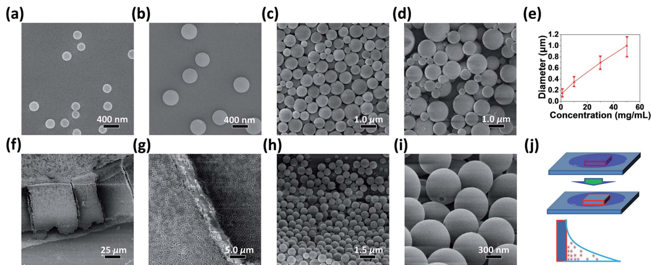
Fig. 1 SEM images of the PPF0H-based CPSMs. PPF0H CPSMs obtained at different initial concentrations in DMF solution: (a) 1 mg mL -1 , (b) 10 mg mL -1 , (c) 30 mg mL -1 , (d) 50 mg mL -1 . (e) Diameter as a function of the concentrations. (f–i) SEM images of three-dimensional (3D) colloidal crystals of PPF0H CPSMs. (j) Schematic representation of PPF0H photonic crystal on silicon substrates fabricated by droplet-pinned solvent evaporation method.
