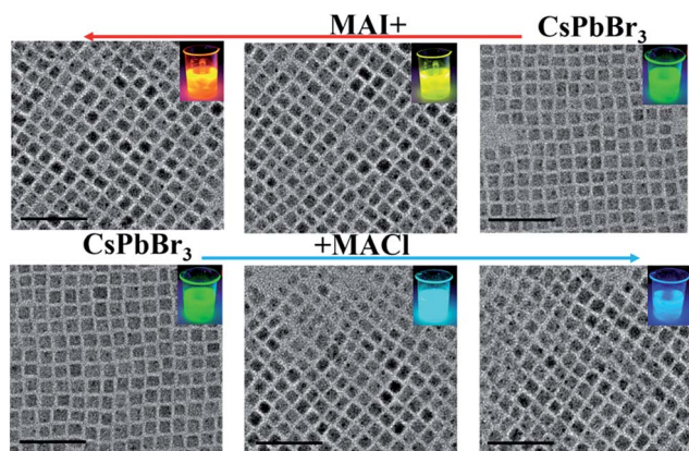
Fig. 4 TEM images of the \text{CsPbBr}_3 NCs after treatment with various quantities of MAI (up) and MACl (down). The insets show the evolution of emission colors (under a UV lamp, \lambda_{\text{ex}} = 365 nm) from crude \text{CsPbBr}_3 NCs to composited perovskite NCs. Scale bars correspond to 50 nm.
