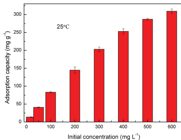
Fig. 6 The effect of initial concentrations (20, 50, 100, 200, 300, 400, 500, 600 \text{ mg L}^{-1} ) on U(VI) removal by PAA hydrogels. (Volume, 10 mL; adsorbent dose, 0.01 g; pH value, 4.0; contact time, 180 min; temperature, 25 \text{ }^\circ\text{C} ; rotating speed, 150 rpm.)
