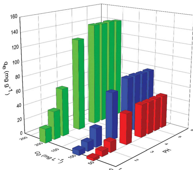
Fig. 5 The effect of initial solution pH on U(VI) removal by PAA hydrogels at various initial concentrations (60, 100 and 200 \text{ mg L}^{-1} ). (Volume, 10 mL; adsorbent dose, 0.01 g; pH value, 1, 1.5, 2, 3, 4, 4.5, 5, 5.5; contact time, 180 min; temperature, 25 \text{ }^\circ\text{C} ; rotating speed, 150 rpm). Note: data are presented as the mean \pm standard deviation of triplicate experiments.
