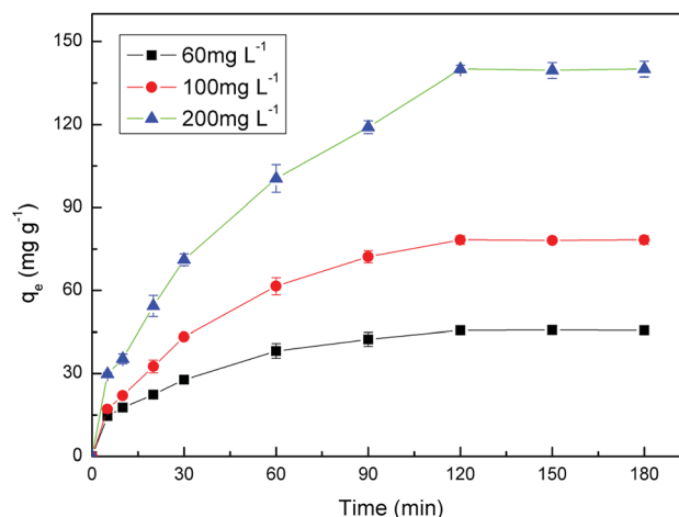
Fig. 7 Effect of contact time on U(VI) adsorption. (Volume, 30 mL; adsorbent dose, 0.03 g; initial concentration, 60, 100 and 200 \text{ mg L}^{-1} ; pH value, 4.0; contact time, 0, 5, 10, 20, 30, 60, 90, 120, 150, 180 min; temperature, 25 \text{ }^\circ\text{C} ; rotating speed, 150 rpm.)
