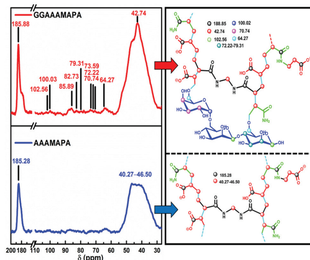
Fig. 4 Solid state ^{13}\text{C} NMR of AAAMAPA and GGAAAMAPA.
