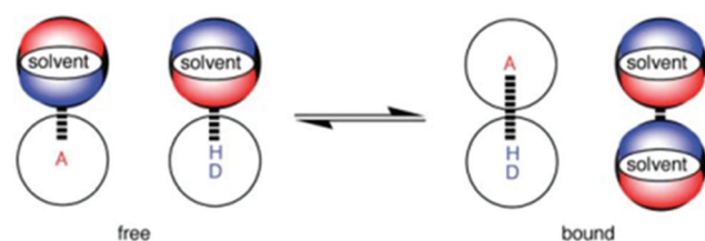
Fig. 1 The solvent competition model for the formation of a H-bonded complex between two solutes. The position of equilibrium is determined by the free energies of the solute-solvent interactions in the free state, and the solute-solute and solvent-solvent interactions in the bound state. A represents a hydrogen-bond acceptor solute and DH a hydrogen-bond donor solute.
