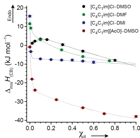
Fig. 9 Relationship between x_{IL} and the heat of cellobiose mixing, \Delta_{mix}H_{(CB)} , for OES solvents derived from [C_4C_1im]Cl or [C_4C_1im][OAc] with DMSO, DMI or DMF. Measurements were obtained at 25 °C. Adapted with permission from ChemSusChem , 2015, 8 , 1577–1584. Wiley-VCH Verlag GmbH & Co. KGaA, 2015.
