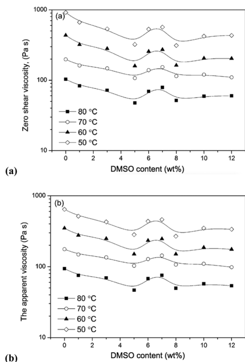
Fig. 11 Influence of DMSO content (wt%) on zero-shear-rate viscosity, (a), and apparent viscosity at shear rate 1 s -1 , (b), for [C 4 C 1 im]Cl–DMSO–cellulose ternary mixtures (5 wt% cellulose), at 50–80 °C (solid lines are provided to guide eyes). Adapted from ref. 126 with permission from the Royal Society of Chemistry.
