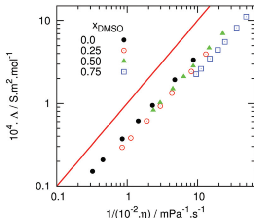
Fig. 8 Walden plot comparing the viscosity and conductivity values for binary [C_4C_1im][OAc] -DMSO mixtures ( x_{DMSO} = 0, 0.25, 0.5, 0.75 ), reproduced from ref. 107 with permission from the Royal Society of Chemistry. The red line denotes the reference ionicity of 0.01 M aqueous KCl, at 25 °C.
