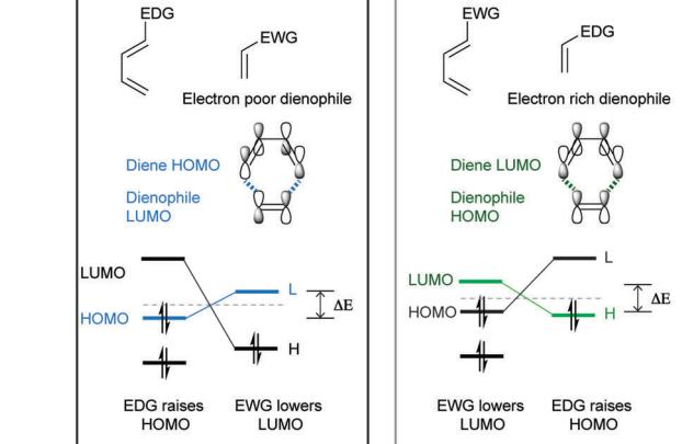
Fig. 4 Mechanism of IEDDA reaction. (a) Schematic representation of the reaction between a dienophile and a tetrazine. (b) Frontier molecular orbital of normal and inverse electron demand Diels–Alder reaction. EDG = electron-donating group, EWG = electron-withdrawing group.
