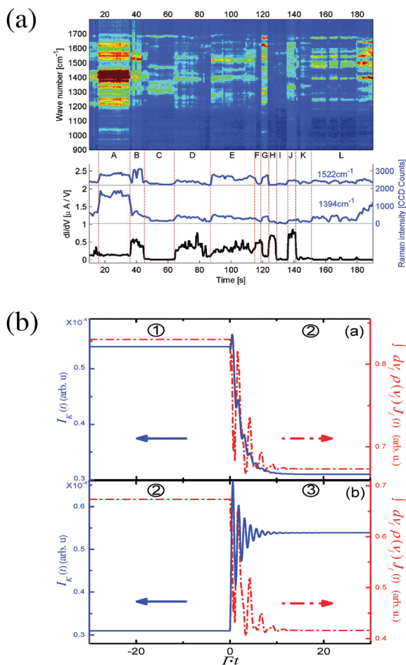
Fig. 7 Time-dependent fluctuations in simultaneously measured electro- nomic conductance and Raman response in molecular junctions. Shown are (a) experimental data and (b) a theoretical analysis. (a) Reprinted with permission from D. R. Ward, N. J. Halas, J. W. Ciszek, J. M. Tour, Y. Wu, P. Nordlander and D. Natelson, Nano Lett. , 2008, 8 , 919–924. Copyright (2008) American Chemical Society. (b) Reprinted with permission from [T.-H. Park and M. Galperin, Phys. Rev. B: Condens. Matter Mater. Phys. , 2011, 84 , 075447.] Copyright (2011) by the American Physical Society. http://dx.doi.org/10.1103/PhysRevB.84.075447 .
