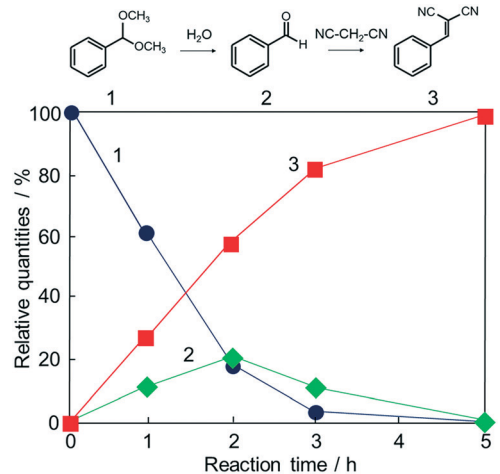
Fig. 6 Time course of the one-pot deacetalization–Knoevenagel condensation reaction over \text{Fe}_3\text{O}_4@HKUST-1 ; benzaldehyde dimethylacetal (1, ●), benzaldehyde (2, ◆), benzylidene-malononitrile (3, ■).
