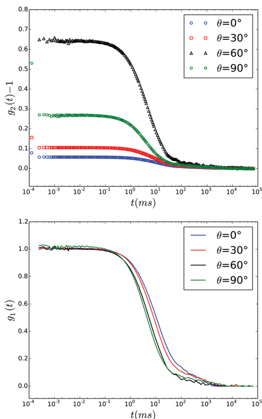
Fig. 2 Time auto correlation functions recorded during a Q_{\parallel} scan in EWDLS at x_r = 60^\circ and values of \theta as indicated in the legend. Top: Intensity correlation functions \hat{g}_2(t) - 1 as measured. Bottom: Field correlation functions calculated by the generalized Siegert relation, eqn (1).
