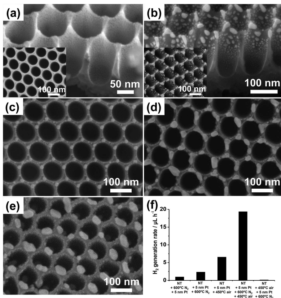
Fig. 11 (a–e) SEM images of TiO_2 nanocavity arrays: (a) sputter-coated with a 5 nm-thick Pt film and (b) after thermal dewetting in N_2 (600 °C); (c–e) sputter-coated with different Pt amounts ((c) 2, (d) 7, and (e) 10 nm) and then dewetted in N_2 . Insets in (a) and (b): top view SEM images. (f) Photocatalytic H_2 generation rate ( r_{H_2} ) of various Pt/ TiO_2 nanocavity arrays decorated by sputtering–dewetting of different Pt loadings. Fig. (a–f) are reprinted (adapted) with permission from ref. 139. Copyright 2016 American Chemical Society.
