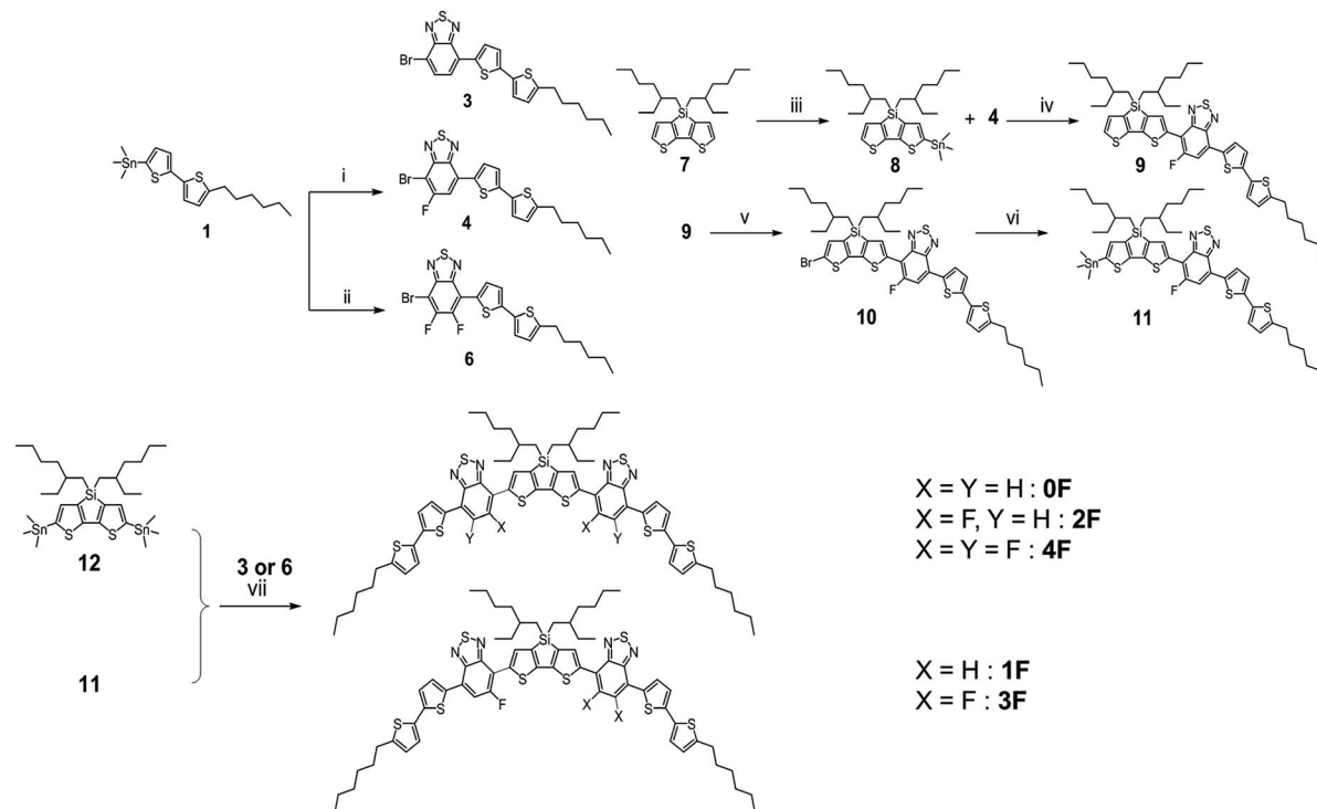
Scheme 1 Synthetic procedure used to prepare 0F , 1F , 2F , 3F , and 4F : (i) \text{Pd}[\text{PPh}_3]_4 , 4,7-dibromo-5-fluorobenzo[c][1,2,5]thiadiazole ( 2 ), toluene, 80 °C, 40 h. (ii) \text{Pd}[\text{PPh}_3]_4 , 4,7-dibromo-5,6-difluorobenzo[c][1,2,5]thiadiazole ( 5 ), toluene, 160 °C, 1 h, microwave. (iii) n\text{-BuLi} , \text{Me}_3\text{SnCl} , THF, R.T., 12 h. (iv) \text{Pd}[\text{PPh}_3]_4 , toluene, 160 °C, 1 h, microwave. (v) NBS, \text{CHCl}_3 , R.T., 24 h. (vi) \text{Pd}[\text{PPh}_3]_4 , hexamethylditin, toluene, 160 °C, 1 h, microwave. (vii) \text{Pd}[\text{PPh}_3]_4 , toluene, 160 °C, 1 h, microwave.
