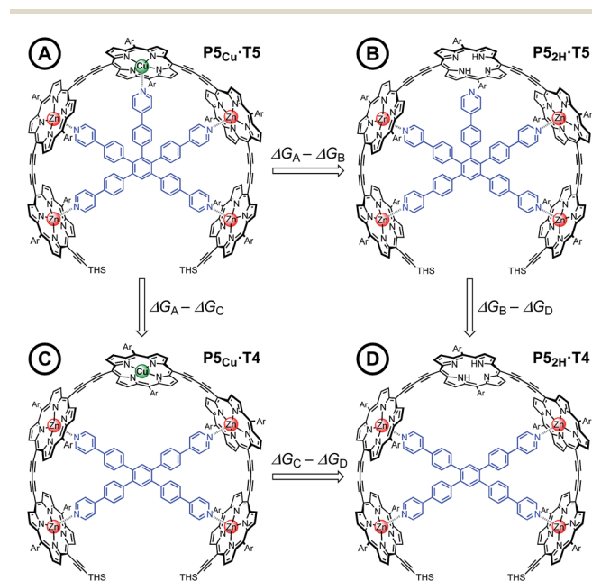
Fig. 4 The chemical DMC used to investigate the interaction between the copper center in the central porphyrin and the pyridine leg of template T5 . Ar = 3,5-bis( tert -butyl)phenyl, THS = trihexylsilyl.
