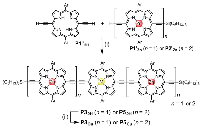
Scheme 1 Synthetic route of \text{P}3_{\text{Cu}} and \text{P}5_{\text{Cu}} . Reaction conditions: (i) \text{Pd}_2(\text{dba})_3 , tri-2-furylphosphine, 1,4-benzoquinone, toluene/ \text{Et}_3\text{N} , 39%; (ii) \text{Cu}(\text{OAc})_2 \cdot \text{H}_2\text{O} , \text{CHCl}_3 , 95%. Ar = 3,5-bis( tert -butyl)phenyl, M = 2H or Cu.
