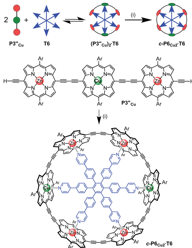
Scheme 2 Synthesis of c\text{-P}6_{\text{Cu}2} \cdot \text{T}6 . Two representations of the synthetic route used to prepare c\text{-P}6_{\text{Cu}2} \cdot \text{T}6 . Reaction conditions: (i) \text{PdCl}_2(\text{PPh}_3)_2 , CuI, 1,4-benzoquinone, i - \text{Pr}_2\text{NH} , \text{CHCl}_3 , 2%. Ar = 3,5-bis( tert -butyl)phenyl.
