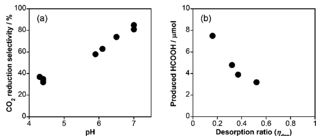
Fig. 4 (a) Selectivity of CO 2 reduction ( \text{sel}_{\text{CO}_2} ) vs. pH of the reaction solution in the photocatalytic reactions. (b) Produced amount of HCOOH vs. desorption ratio of RuRu ( \eta_{\text{des}} ) by the photocatalytic reactions with various concentration of NaH 2 PO 4 (pH = 4.4).
