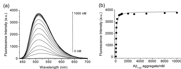
Fig. 3 (a) Change in fluorescence intensity and (b) the fluorescence titration curve for the complexation of QAD1 (1 \mu M ) with A \beta_{1-42} aggregates (0–10 \mu M ) in PBS buffer (10 mM, pH 7.4). The calculated value is represented by a solid line. The excitation wavelength was 407 nm and the fluorescence intensity was measured at 510 nm.
