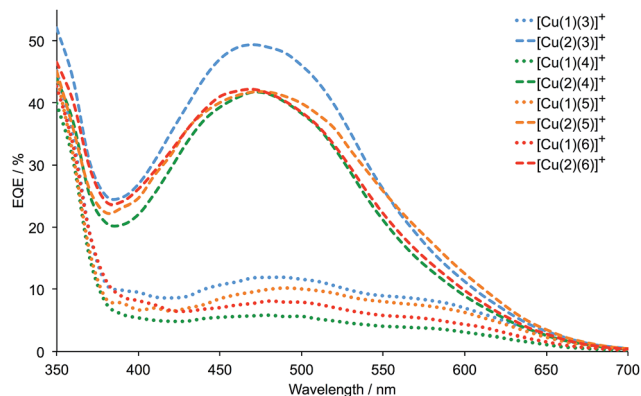
Fig. 7 EQE spectra for DSCs containing the dyes [Cu(1)(L_{ancillary})]^+ and [Cu(2)(L_{ancillary})]^+ ( L_{ancillary} = 3-6 ) measured on the day the DSCs were made.
