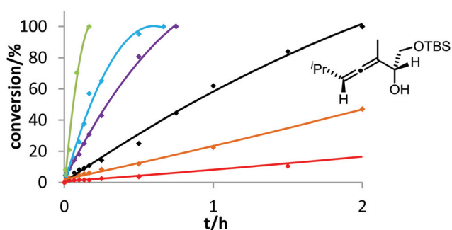
Fig. 1 Ligand effect on the gold-catalyzed cycloisomerization of 3a . 4 mol% [Au] and 4 mol% AgOTf were used in DMF at room temperature. Decreasing reactivity was observed in the following order: B (green) > (4-MeOC 6 H 4 ) 3 PAuCl (blue) > (4-MeC 6 H 4 ) 3 PAuCl (violet) > Ph 3 PAuCl (black) > (4-CF 3 C 6 H 4 ) 3 PAuCl (orange) > D (red).
