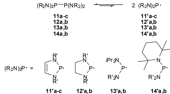
Scheme 13 P–P bond dissociation equilibria for tetraamino-diphosphines (R' = tBu ( 11a ), 2,6-Me 2 C 6 H 3 ( 11b ), 2,6-iPr 2 C 6 H 3 ( 11b , 12a ), 2-tBu 2 C 6 H 4 ( 12b ), iPr ( 13a , 14b ), SiMe 3 ( 13b ), Et ( 14a )).
