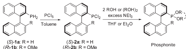
Scheme 1 The synthesis of the phosphonite ligands from (S)-1a and (R)-1b.
