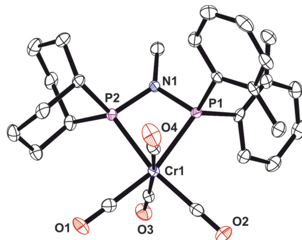
Fig. 9 Crystal structure of [\text{Cr}(\text{CO})_4(L_g)] ( 8 ). All hydrogen atoms have been omitted for clarity. Selected bond lengths (Å) and angles (°): Cr(1)–P(1) 2.3477(6), Cr(1)–P(2) 2.3669(6), P(1)–N(1) 1.7146(17), P(2)–N(1) 1.7035(17), P(1)–Cr(1)–P(2) 68.04(4), P(2)–N(1)–P(1) 101.01(9), N(1)–P(1)–Cr(1) 94.67(6), N(1)–P(2)–Cr(1) 94.29(6), C(16)–P(1)–C(13) 95.66(10), C(7)–P(2)–C(4) 105.17(9).
