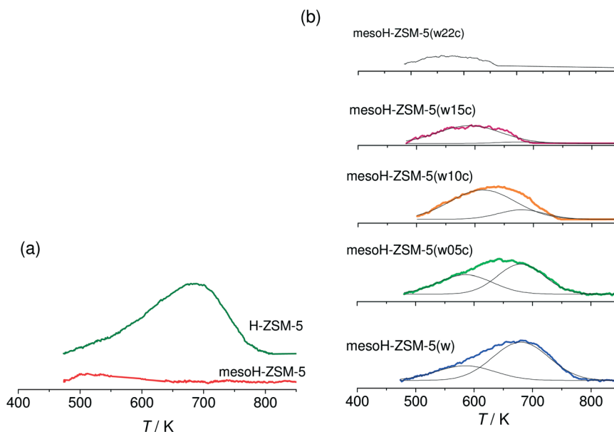
Fig. 4 \text{NH}_3 -TPD profiles ( 10 \text{ K min}^{-1} ) of the micro- and mesoporous zeolites (a) and the acid washed and carbon/zeolite composites (b). \text{NH}_3 was adsorbed at 473 K.
