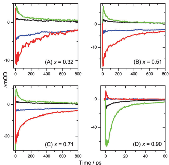
Fig. 5 Kinetic traces extracted from transient PSCP broadband absorption spectra for (\text{MAI})_x(\text{PbI}_2)_{1-x}/\text{TiO}_2/\text{glass} samples. Panels (A–D) are for x = 0.32, 0.51, 0.71 and 0.90 , respectively. Black and green lines are for 2 and 50 \mu\text{J cm}^{-2} fluence at \lambda_{\text{probe}} = 600 nm. Blue and red lines represent 2 and 50 \mu\text{J cm}^{-2} fluence at \lambda_{\text{probe}} = 750 nm.
