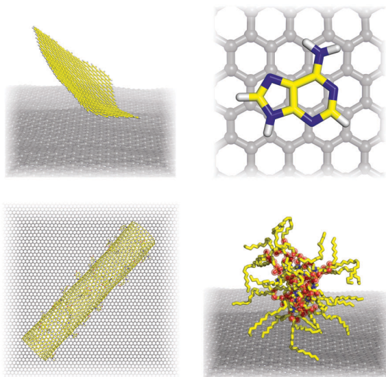
Fig. 7 Screenshots from molecular dynamics simulations of various processes taking place on a graphene surface: graphene exfoliation (top left), nucleobase adsorption (top right), graphene-carbon nanotube assembly (bottom left), and the formation of a reverse lecithin micelle on a graphene surface.
