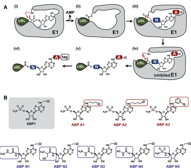
Fig. 2 Mechanistic considerations in the design of selective inhibitors of E1 enzymes. (A) Mechanism of ABP1 analogue-mediated E1 inhibition (B) Structures of proposed ABP1 analogues.
