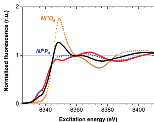
Fig. 4 X-ray absorption near edge structure spectra (Ni K edge) of the Ni-CNT material as prepared (black solid line), and after 1 h H_2 oxidation (red solid line). Spectra of pristine [Ni(P^{Ph}N_2CH_2pyrene)_2] (blue dotted line) and of [Ni^{II}(OH_2)_6]^{2+} (orange dotted line) are shown for comparison. See Fig. S10† for a magnification of the K edge region.
