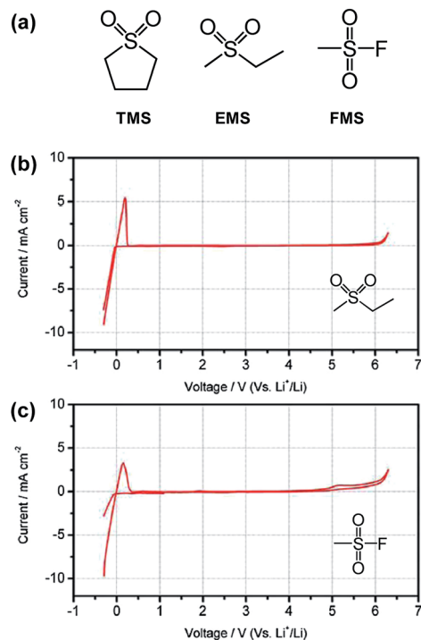
Fig. 14 (a) Structures of typical sulfone solvents. Cyclic voltammograms of 1 M \text{LiPF}_6 in (b) EMS/DMC (1 : 1 by wt) and (c) EMS/FMS (1 : 1 by wt). Scan rate: 5 \text{mV s}^{-1} . Pt as the working and counter electrodes and Li as the reference electrode. Reproduced with permission. 78
