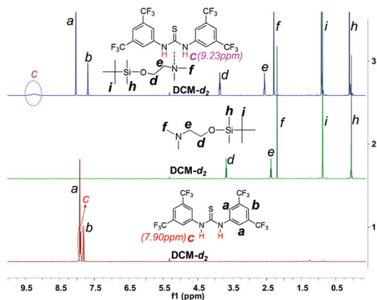
Fig. 3 Expanded ^1\text{H} NMR spectra of TU-S, DMEA-TMS' and TU-S/DMEA-TMS' (1:1) mixture (500 M, 25 ^\circ\text{C} , \text{CD}_2\text{Cl}_2 , for full spectra see Fig. S6 and S7 \dagger ).
