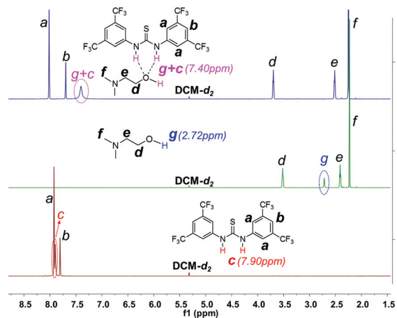
Fig. 5 ^1\text{H} NMR spectra of TU-S, DMEA and TU-S/DMEA (1:1) mixture (500 M, 25 ^\circ\text{C} , \text{CD}_2\text{Cl}_2 , for full spectra see Fig. S12 \dagger ).
