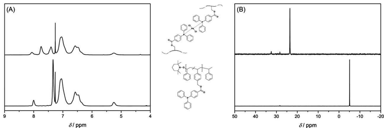
Fig. 1 Intramolecular crosslinking by metal–ligand complexation monitored by ^1\text{H} NMR (A) and ^{31}\text{P}\{^1\text{H}\} NMR spectroscopy (B) in \text{CDCl}_3 at 25^\circ\text{C} . The complete shift of the proton and phosphorus resonances indicates quantitative complexation (the crosslinking chemistry presents a schematic view, in which we suggest a trans -configuration of the Pd-atoms, see text).
