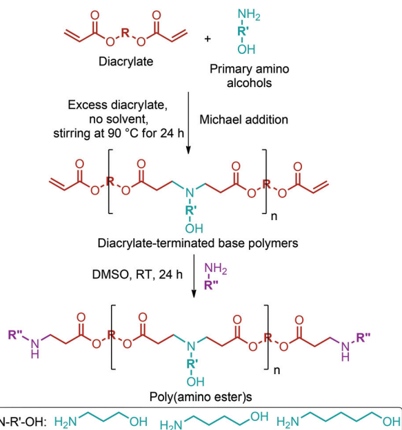
Fig. 18 Synthesis of the poly(β-amino ester) library. Adapted from ref. 306.
