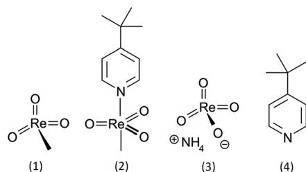
Fig. 1 Structures of the compounds investigated in detail (test set 1): (1) methyltrioxorhenium (MTO), (2) (4- tert -butylpyridine)-methyltrioxorhenium (MTO-TBP), (3) ammonium perrhenate ( \text{NH}_4\text{ReO}_4 ), (4) 4- tert -butylpyridine (TBP).
