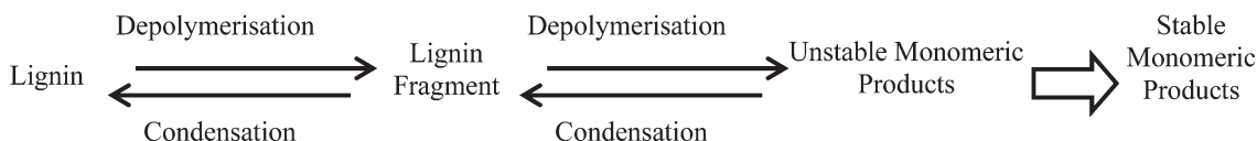
Fig. 7 Lignin depolymerisation/condensation scheme.
