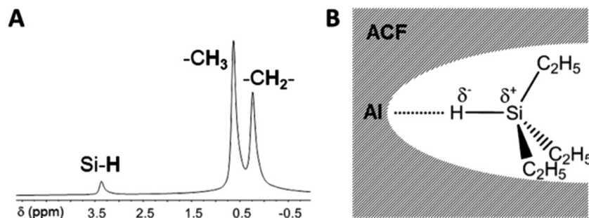
Fig. 14 (a) 1 H MAS NMR spectrum showing the signals for surface-bound Et 3 SiH ( \nu_{\text{rot}} = 10 kHz) with the SiH resonance at \delta = 3.45 ppm. For Et 3 SiH in C 6 D 6 solution, the resonance is observed at \delta = 3.85 ppm. (b) Schematic representation of ACF...H-SiEt 3 . Reproduced from ref. 26 with permission of the Royal Society of Chemistry.
