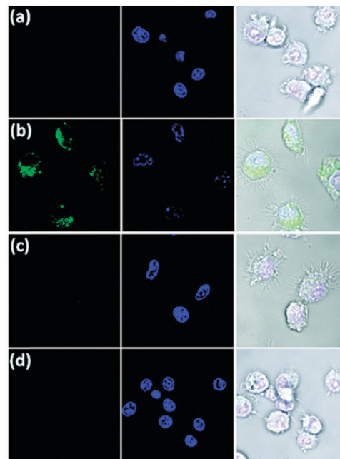
Fig. 69 Top: structure of HKGreen1 , 2 and 3 and reactivity of BODIPY based chemodosimeters HKGreen1 with peroxyxynitrite to form 70 . Bottom: images of live RAW264.7 cells were treated with stimulants to elicit endogenous \text{ONOO}^- production then stained with HKGreen-3 (green channel) and Hoechst 33342 (blue channel). (a) Cells without stimulation. (b) Cells stimulated with LPS, IFN- \gamma , and PMA. (c) Cells pre-treated with TEMPO, and then stimulated with LPS, IFN- \gamma , and PMA. (d) Cells pre-treated with AG, then stimulated with LPS, IFN- \gamma , and PMA. Image reproduced with permission. 92
