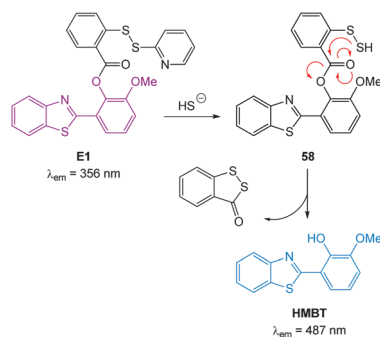
Scheme 1 Structure and reaction mechanism of E1 with HS - .
