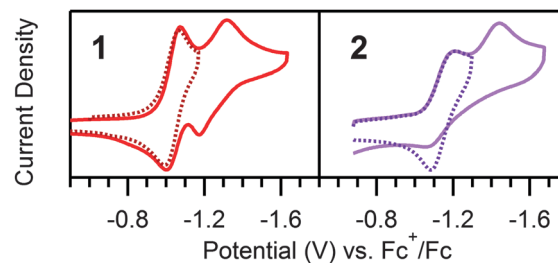
Fig. 2 Cyclic voltammograms of 0.20 mM 1 and 2 without acid at 100 \text{ mV s}^{-1} and with 0.1 M [\text{Bu}_4\text{N}][\text{PF}_6] . The \text{Ni}^{\text{II}}/\text{Ni}^{\text{I}} reduction of 1 is reversible (dotted trace) and the \text{Ni}^{\text{I}}/\text{Ni}^{\text{0}} reduction is quasi reversible. The \text{Ni}^{\text{I}}/\text{Ni}^{\text{0}} reduction of 2 is reversible (dotted trace); however the \text{Ni}^{\text{II}}/\text{Ni}^{\text{I}} reduction is irreversible.
