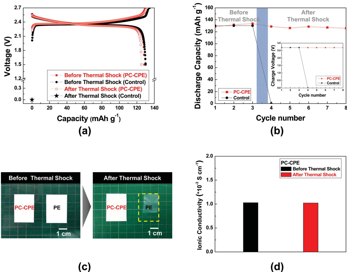
Fig. 6 Thermal stability of Al pouch-type full cells assembled with PC-CPE or carbonate-based liquid electrolyte ( 1 M \text{LiPF}_6 in EC/DMC = 1/1 v/v) and PE separator: (a) variation in charge/discharge profiles of cells after exposure to thermal shock ( \approx 130 °C/ 0.5 h); (b) variation in discharge capacity and charge voltage (inset) of cells before/after the thermal shock. (c) Comparison of thermal shrinkage between PC-CPE and PE separator after exposure to the thermal shock. (d) Ionic conductivity of PC-CPE before/after the thermal shock.
