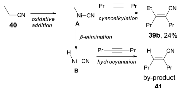
Scheme 21 Formation of the hydrocyanation byproducts in cyanoalkylations.
