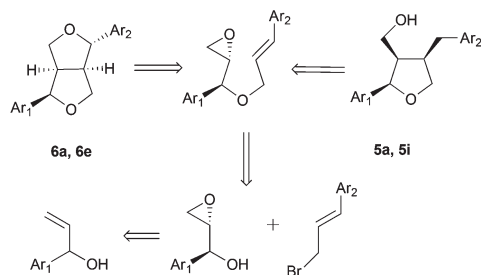
Scheme 27 Retrosynthetic analysis.
