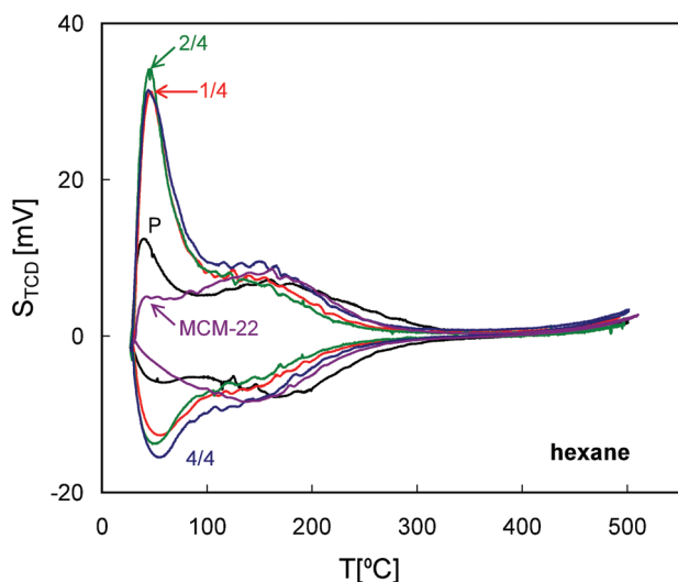
Fig. 10 QE-TPDA profiles of hexane measured for the studied zeolites MCM-56 and MCM-22 at 10 °C min -1 .
