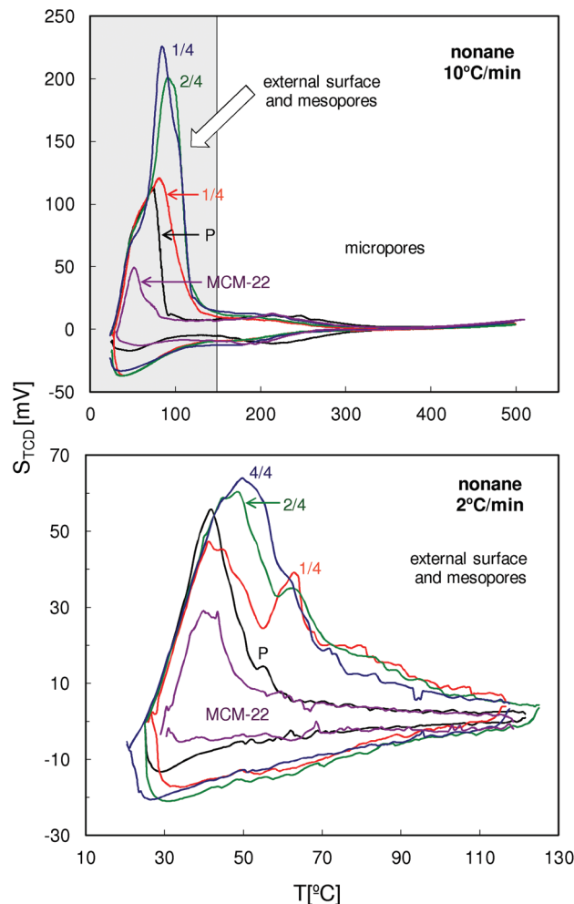
Fig. 11 QE-TPDA profiles of nonane measured for the studied zeolites MCM-56 and MCM-22 at 10 and 2 °C min -1 .
